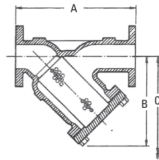
Model 911U
